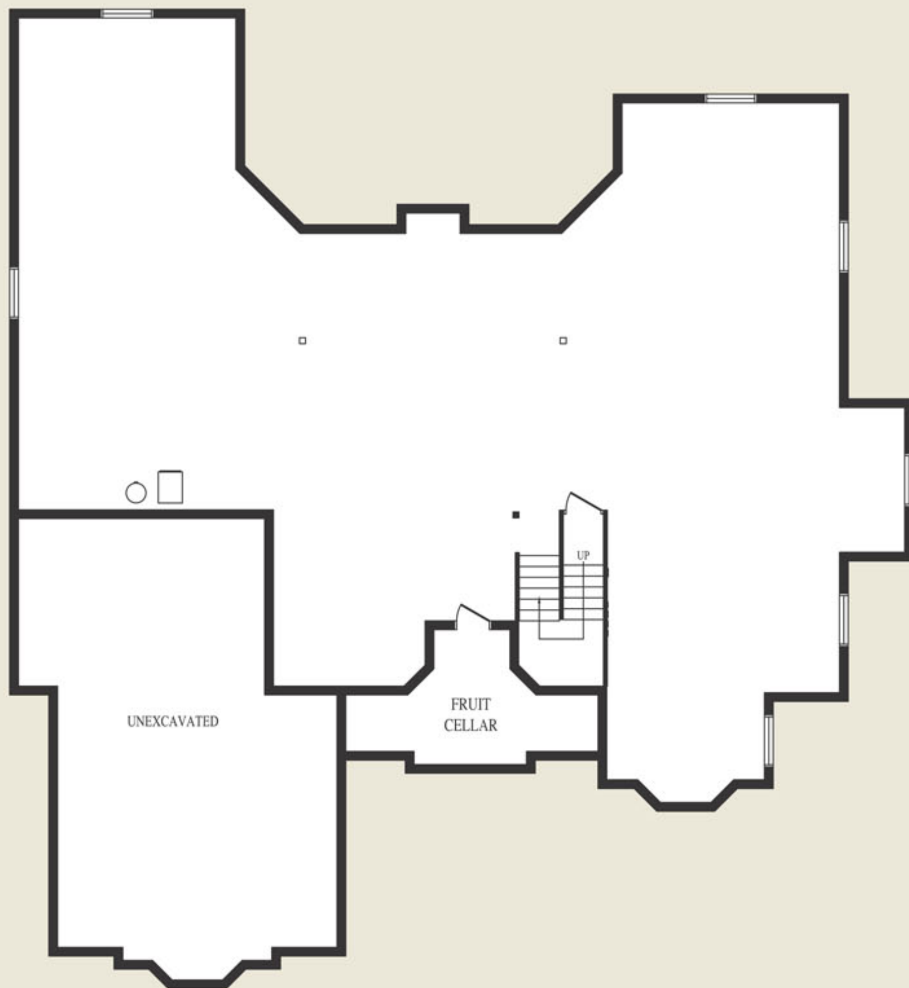
Basement Plan
